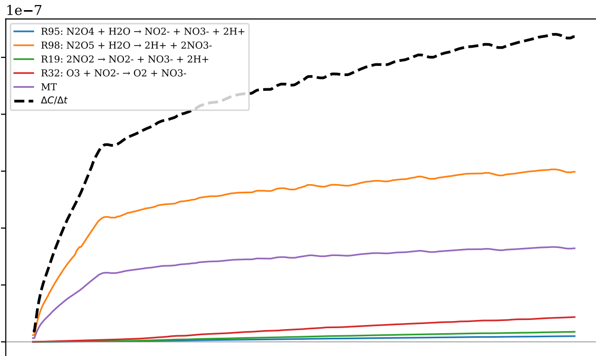
(a) \text{NO}_3^-
