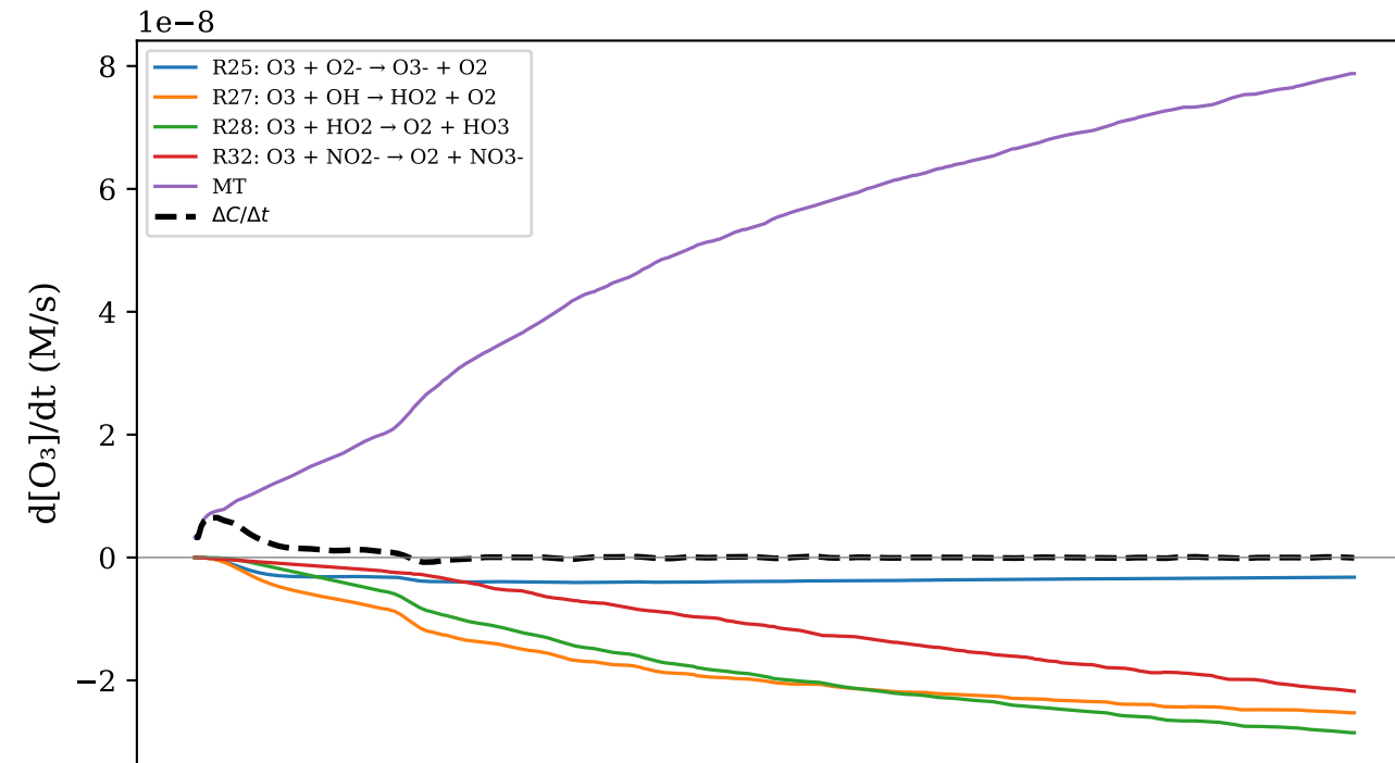
(b) \text{O}_3
